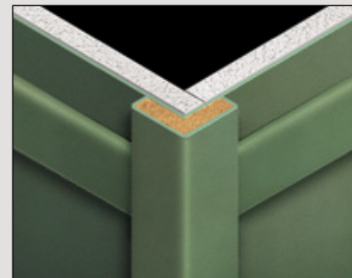
Full Height Outside Corner (5/8" thick) Includes 1/2" thick horizontal trim
