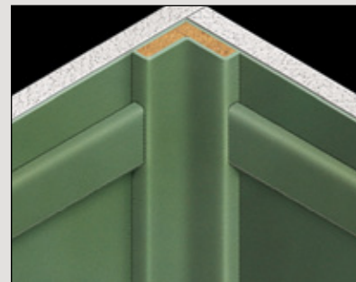
Full Height Inside Corner (5/8" thick) Includes 1/2" thick horizontal trim
