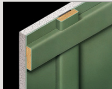
Full Height Vertical/Horizontal Transition Includes 3/8" thick vertical trim and 1/2" thick horizontal trim
