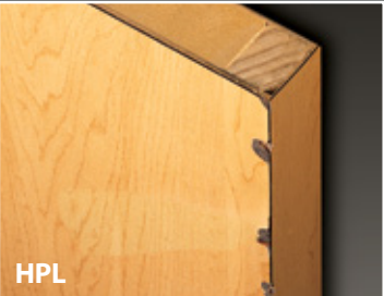
At a 4" drop the HPL laminate chipped, exposing sharp edges.
